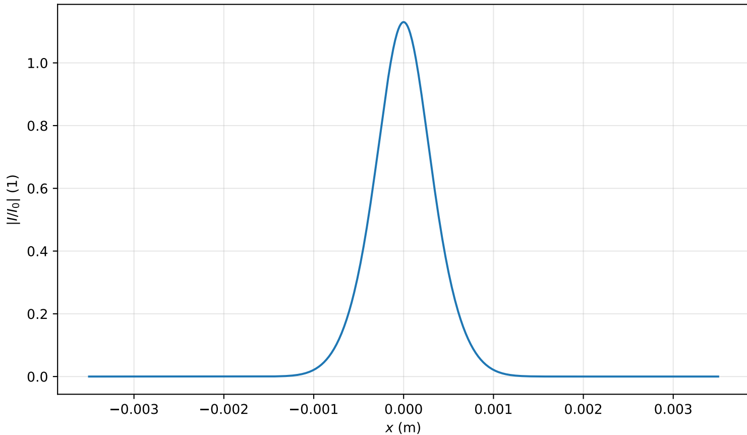
Intensity profile I(x, y = 0, z = 0.637m)/I_0 , P_{in}=0.7P_{cr} , artificial time
